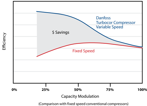
Figure 3: Frictionless design is more efficient over entire range.
