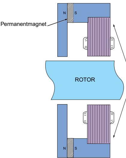
Cross-section of radial bearing
